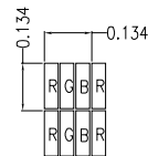
PIXEL DETAIL (SCALE 100:1)
